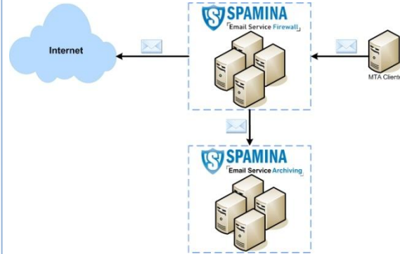
Figure 2. Archiving outgoing mail
